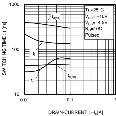
Fig.13 Switching Characteristics
